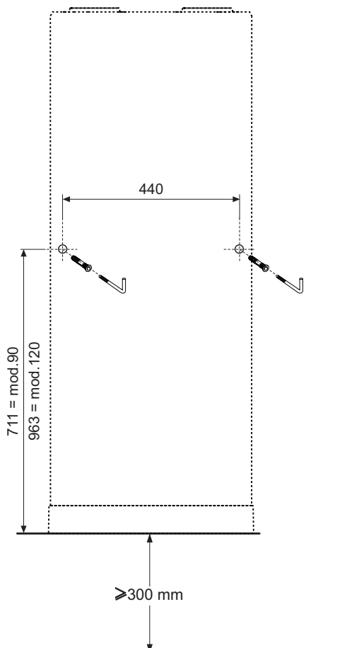
fig. 50 - Drilling indication
